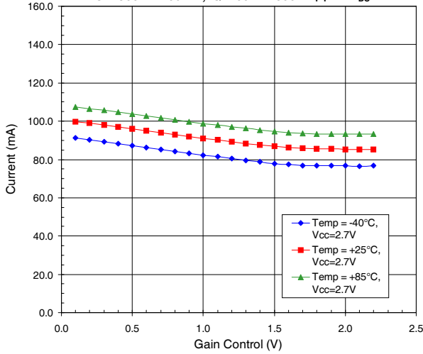
High Band Current Consumption versus Gain Control LO=1900MHz 0dBm, IQ=100kHz 800mV p-p 1.2V DC
